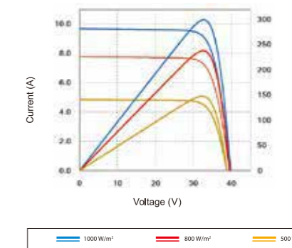
I-V Curves
